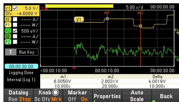
Figure 7. Log data with sample interval 20 μs to 60 s, for up to 10,000 hours or 5 MB of data
